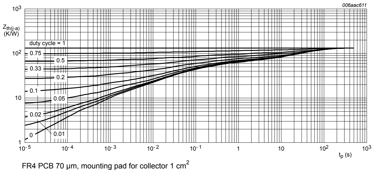
Fig. 7. Per transistor: transient thermal impedance from junction to ambient as a function of pulse duration; typical values
