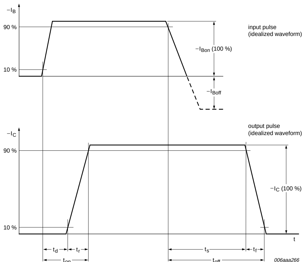
Fig 18. TR1: BISS transistor switching time definition
