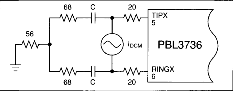
Figure 3. Single-frequency noise test Circuit. \frac{1}{\omega C} \ll 100\text{ ohms}
