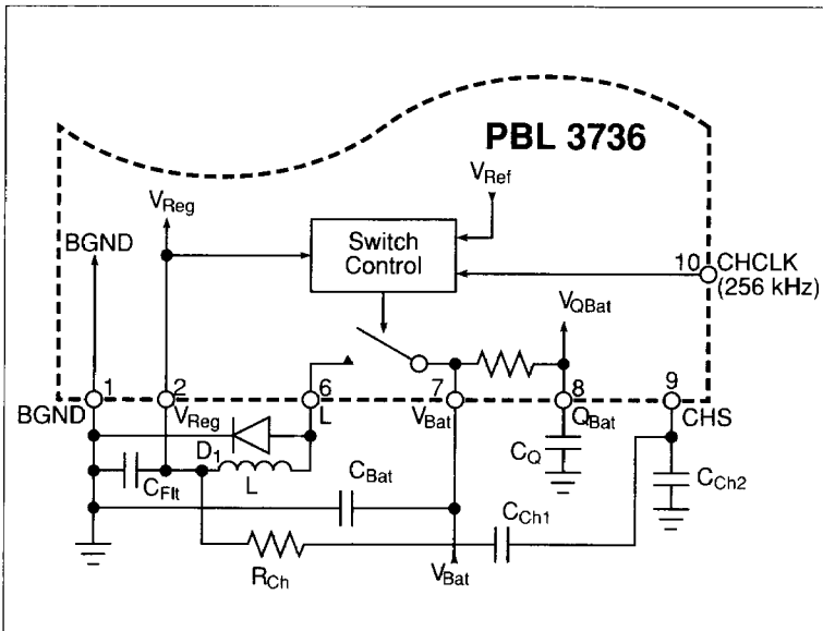
Figure 10. Switching regulator.
