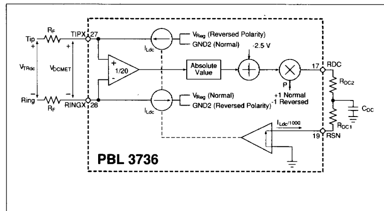
Figure 9. Battery feed.
