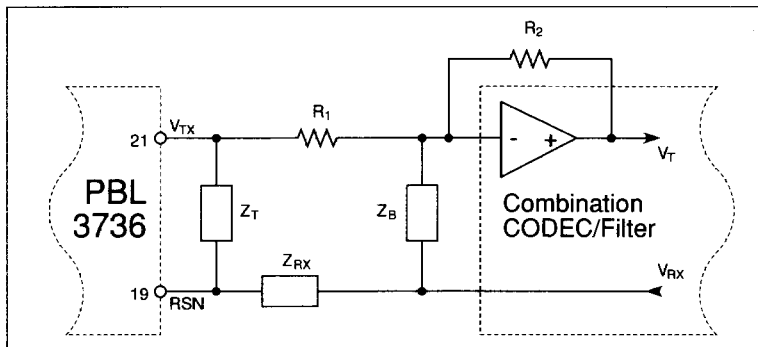
Figure 7. Hybrid function.
