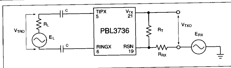
Figure 1. Test circuit for transmission parameters.
