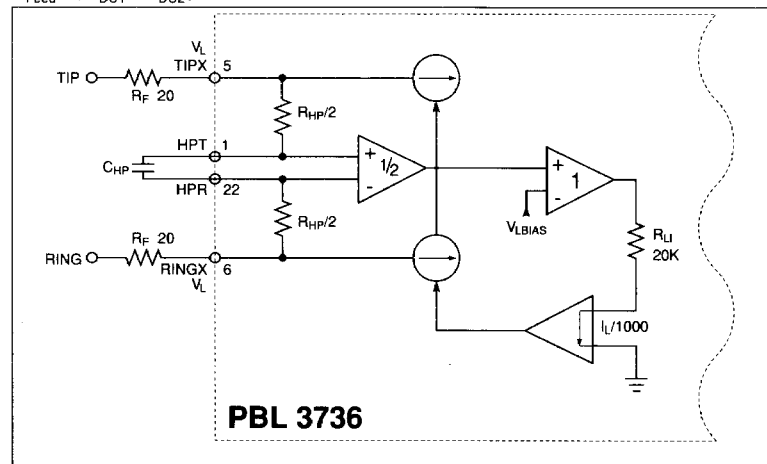
Figure 8. Longitudinal impedance.
