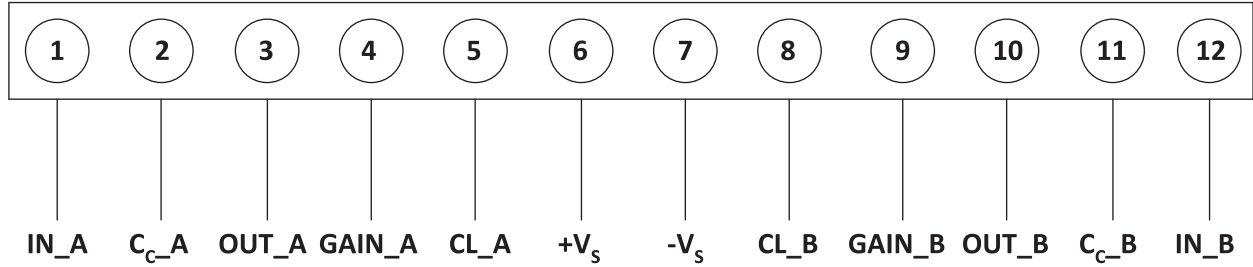
Figure 2: External Connections
