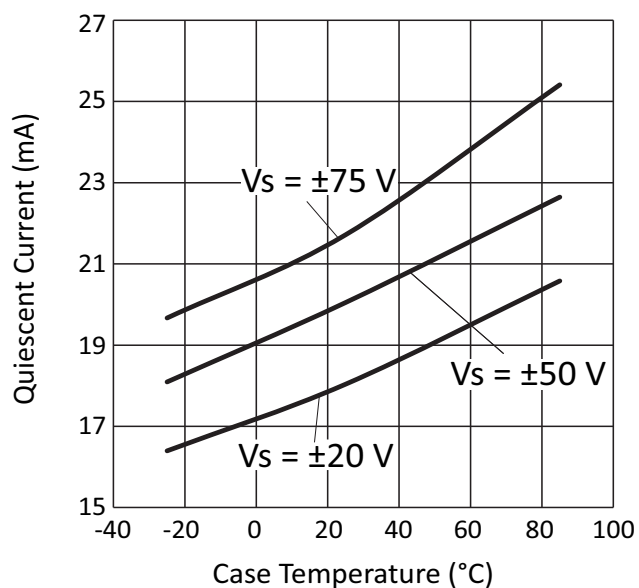
Figure 9: Quiescent Current
