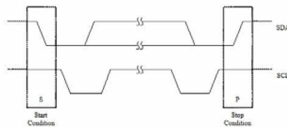
Figure 2.1 Start and Stop conditions
