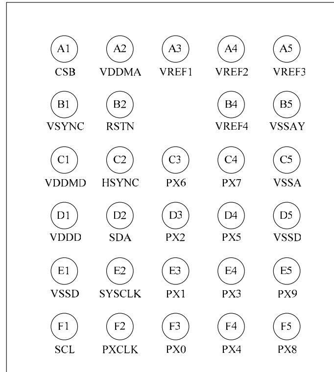
PAS6371LT
