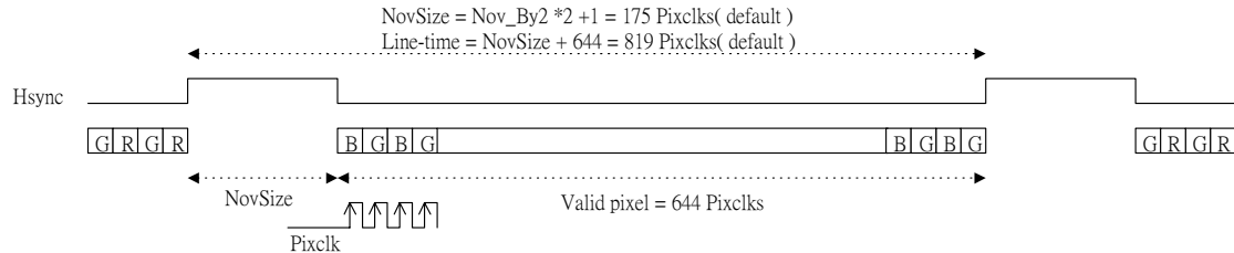
Figure 4.2 Inter-line timing ( default )
