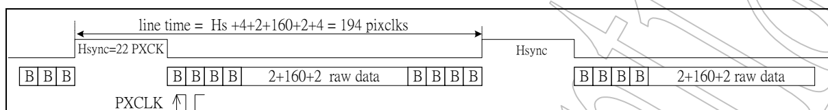
Fig. 4.1 Inter-line timing
