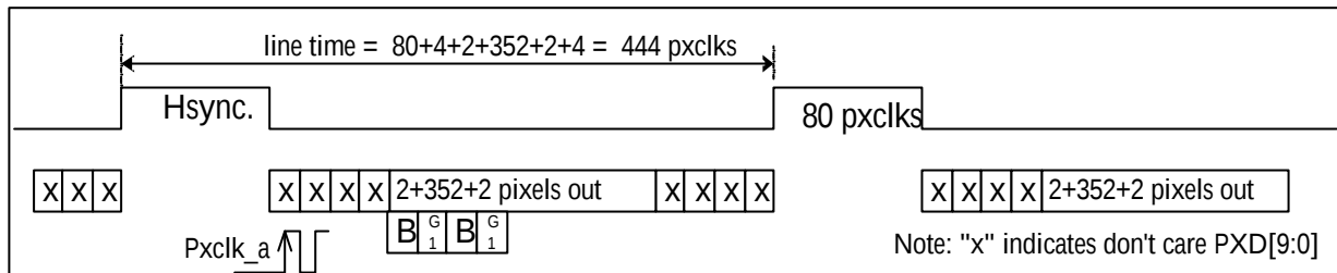
Fig 4.1. Inter-line timing
