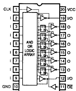
CERDIP CERPACK
