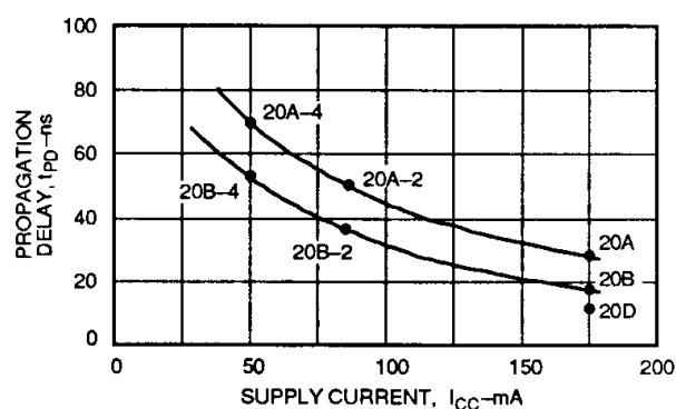
20-Pin PAL Device Speed vs Power
