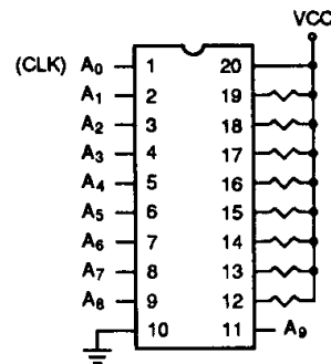
PAL16R8A/B/D PAL16R8A-2/B-2 PAL16R8A-4/B-4
