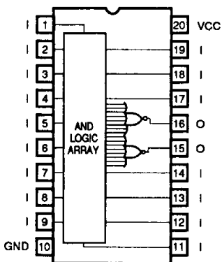
CERDIP CERPACK
