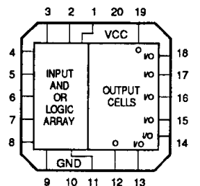
LEADLESS CHIP CARRIER
