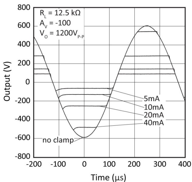
Figure 6: Large Signal Response with Current Limit
