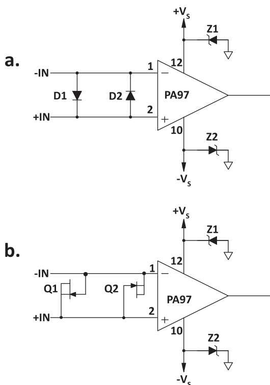
Figure 13: Input Protection
