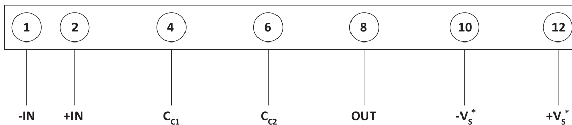
Figure 3: External Connections
