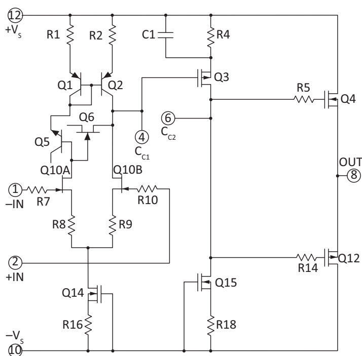
Figure 1: Equivalent Schematic
