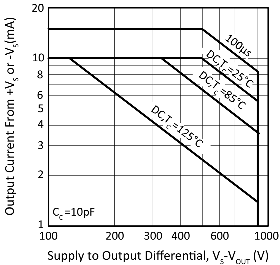
Figure 11: SOA
