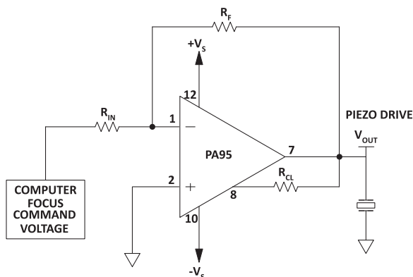
Figure 13: Typical Application
