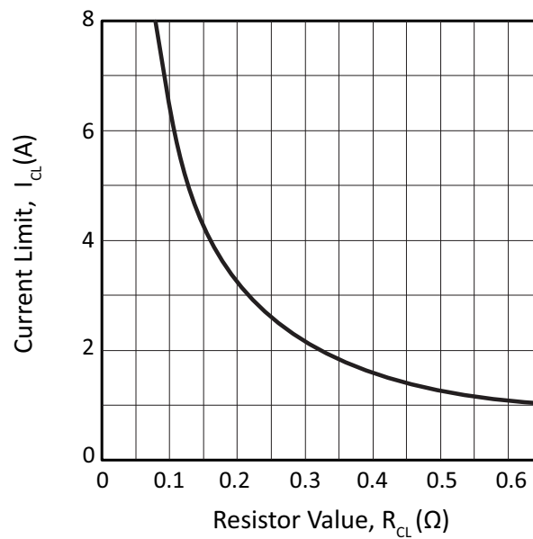
Figure 13: Current Limit
