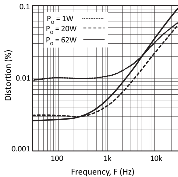
Figure 11: Harmonic Distortion
