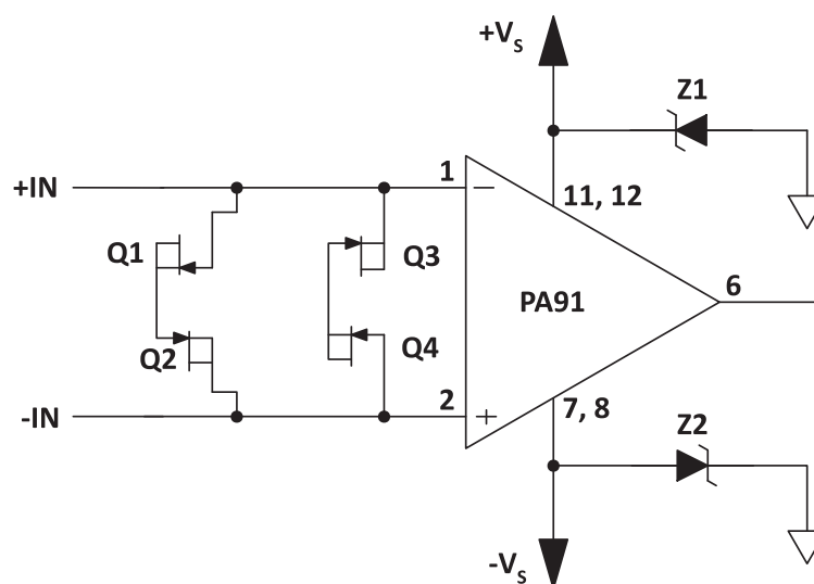
Figure 16: Overvoltage Protection
