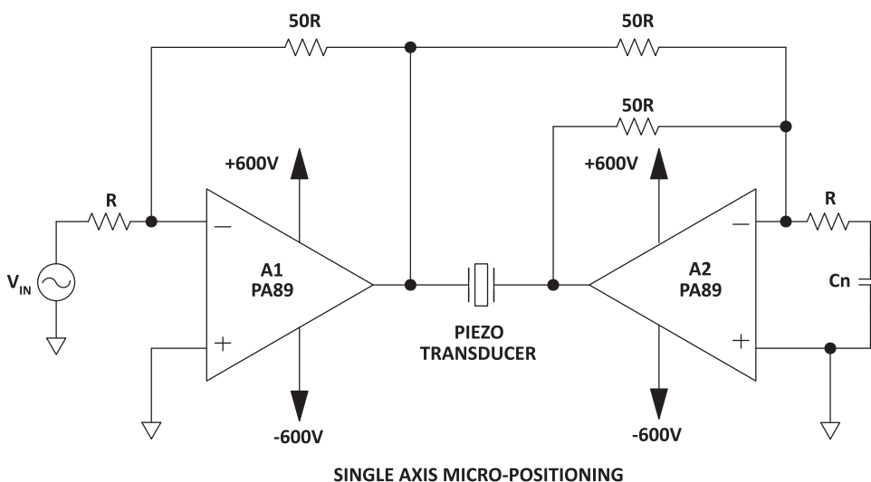
Figure 17: Typical Application
