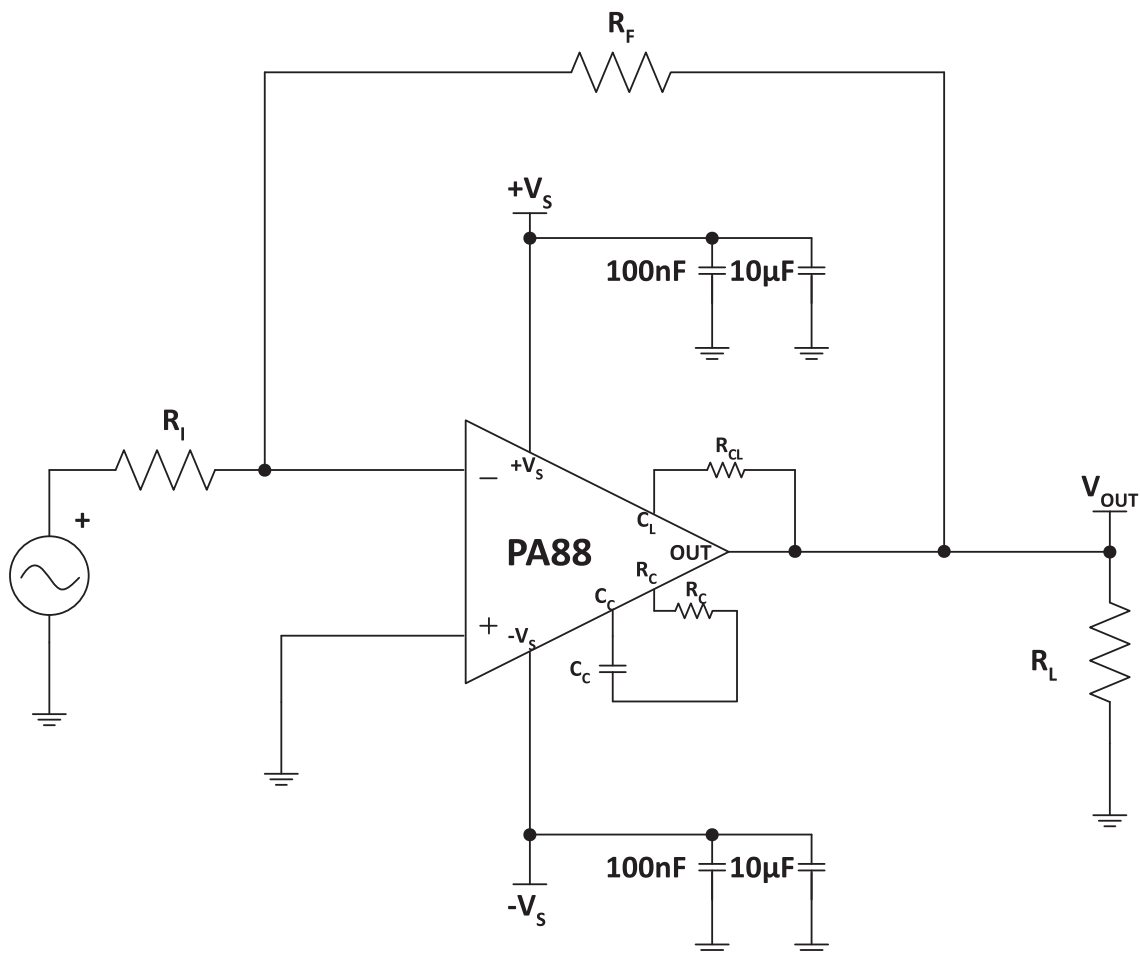
Figure 1: Typical Connection
