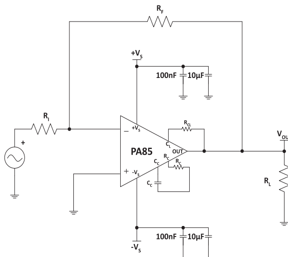
Figure 1: Typical Connection
