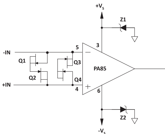
Figure 17: Overvoltage Protection
