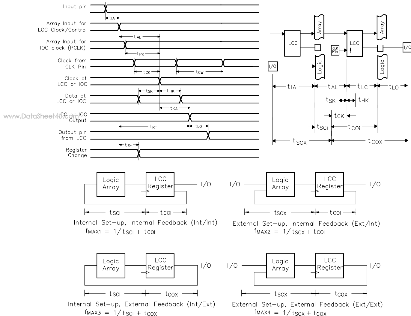
Figure 16. Sequential Timing – Waveforms and Block Diagram
