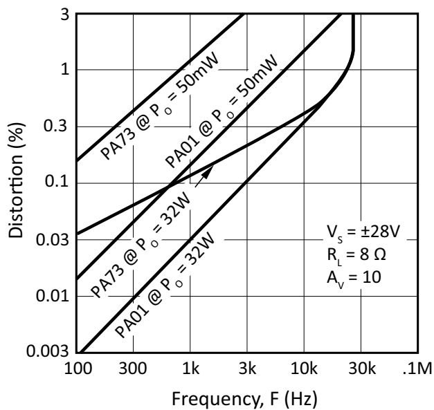
Figure 13: Harmonic Distortion
