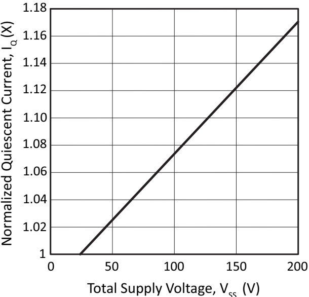
Figure 11: Quiescent Current
