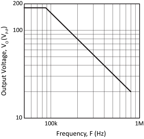
Figure 9: Power Response
