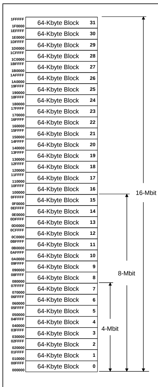
Figure 5. Memory Map
