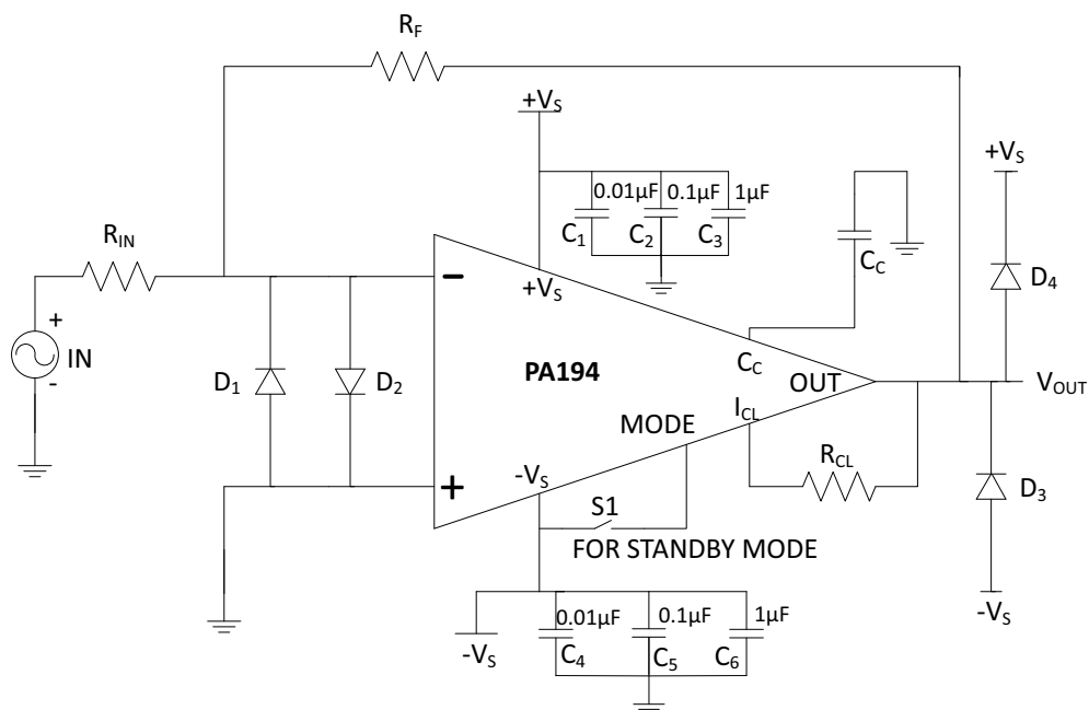
Figure 2: Typical Connection
