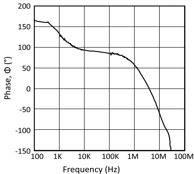
Figure 5: Phase Response, C_C = 0\text{pF}
