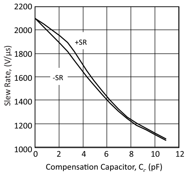
Figure 13: Slew Rate vs. Compensation Capacitor, A_V = -10 \text{ V/V}
