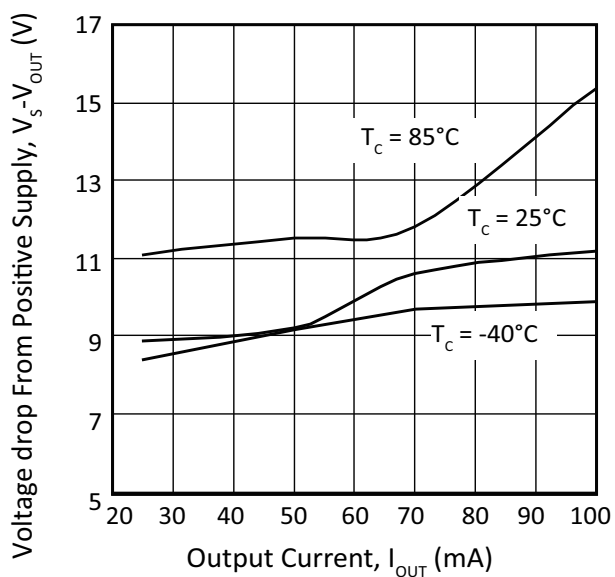
Figure 6: Positive Output Voltage Swing
