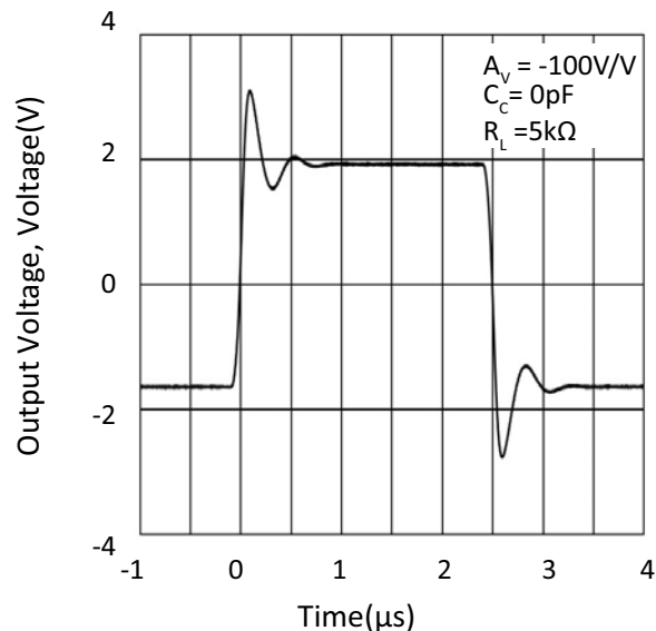
Figure 9: Small Signal Pulse Response
