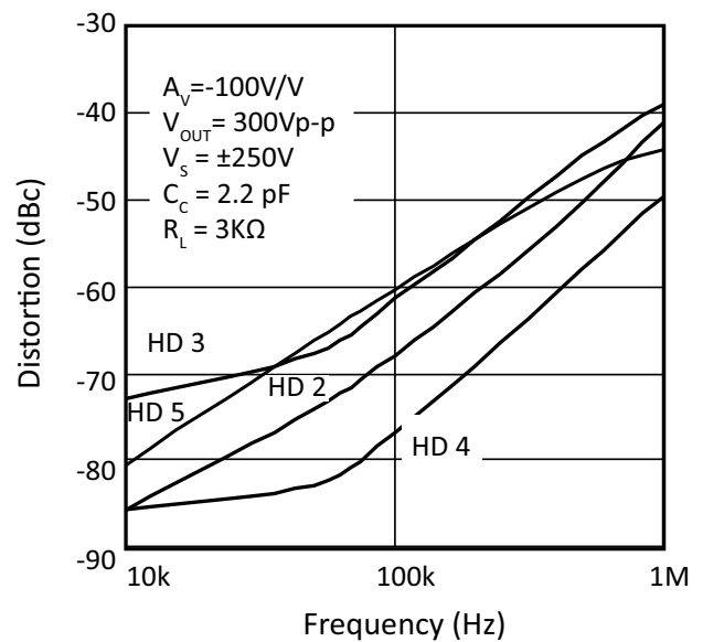
Figure 19: Harmonic Distortion
