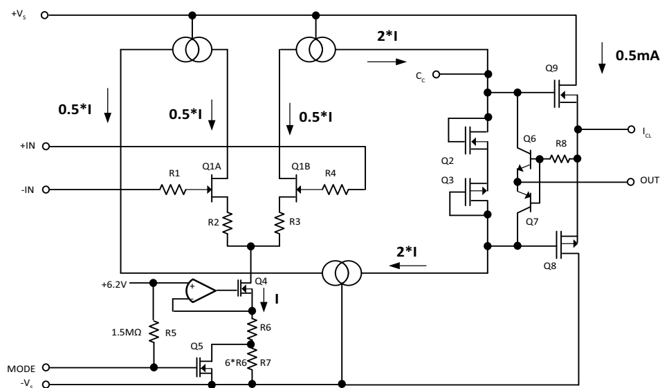
Figure 1: Equivalent Schematic
