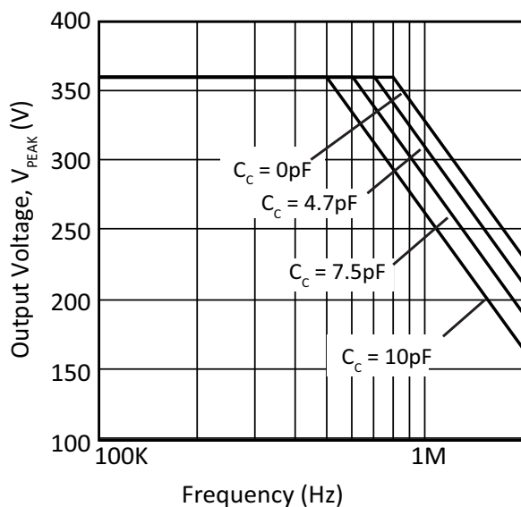
Figure 8: Power Response
