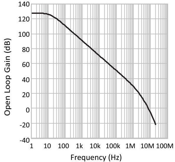
Figure 22: PA165 Open Loop Frequency Response, C_C=0\text{pF}
