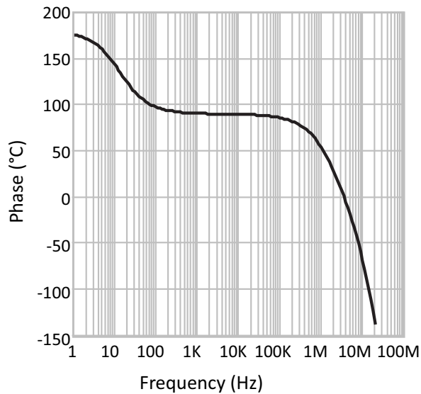
Figure 21: PA165 Open Loop Phase Response, C_C=0\text{pF}
