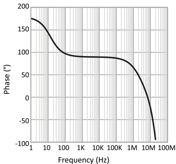
Figure 14: PA164 Open Loop Phase Response, C C = 0pF
