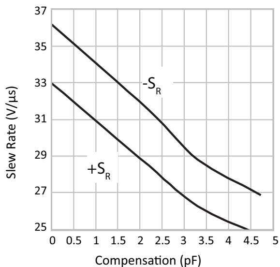
Figure 13: PA164 Slew Rate vs. Compensation
