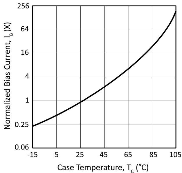
Figure 10: Bias Current
