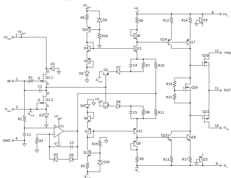
Figure 1: Equivalent Schematic
