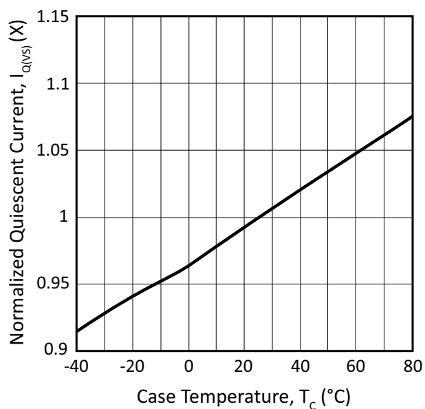
Figure 11: High Voltage Current vs. Temperature
