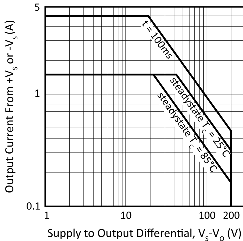
Figure 16: SOA
