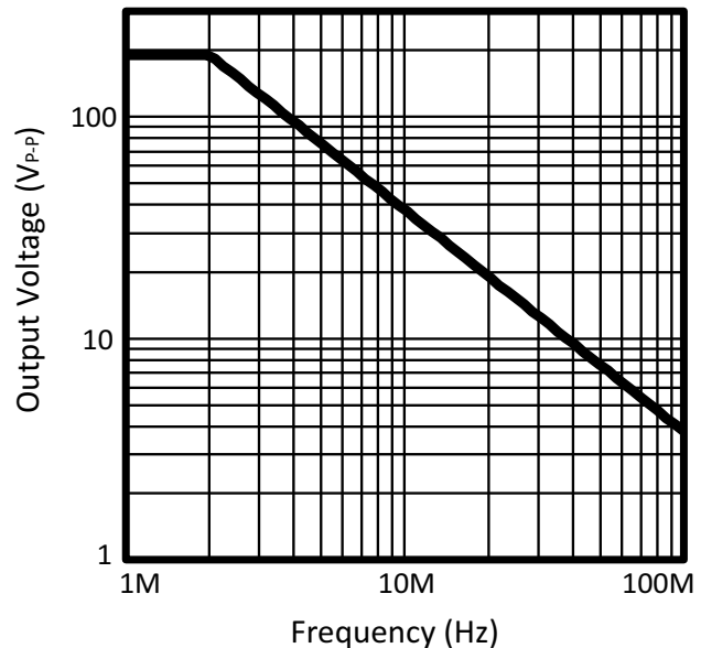
Figure 15: Power Response
