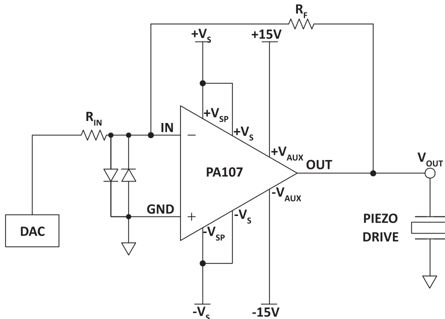
Figure 17: Typical Application
