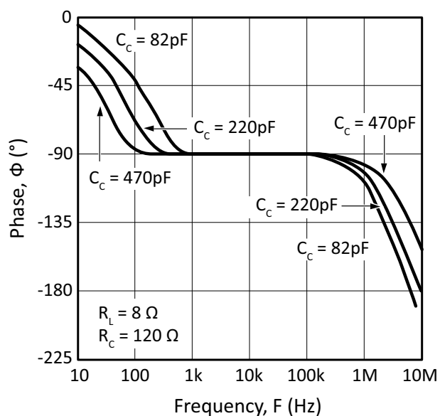
Figure 7: Phase Response
