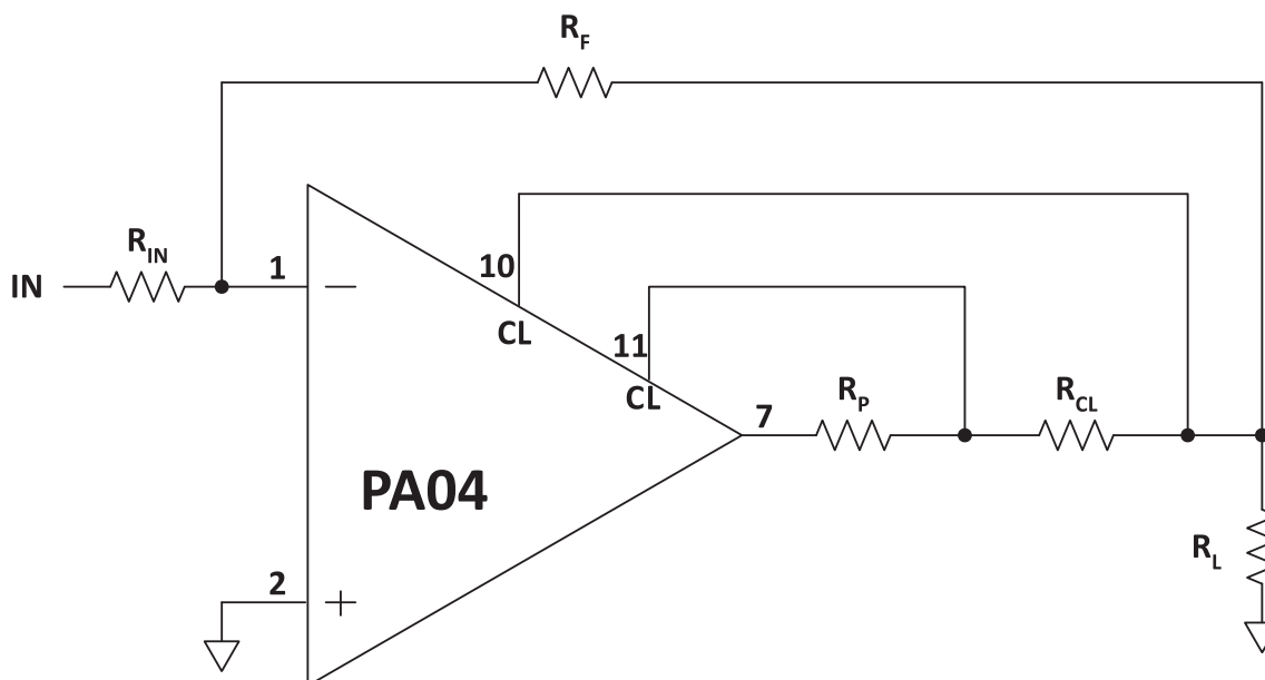
Figure 18: Current Limit
