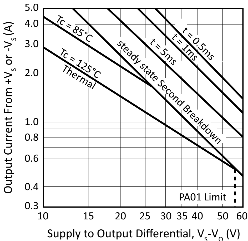
Figure 15: SOA
