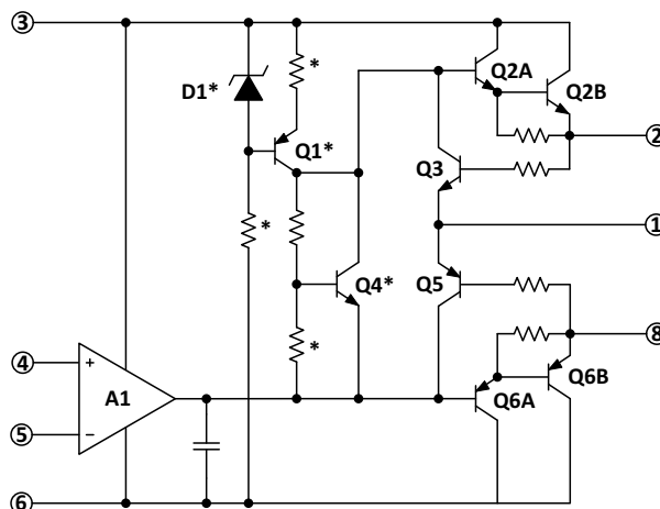
Figure 1: Equivalent Schematic
