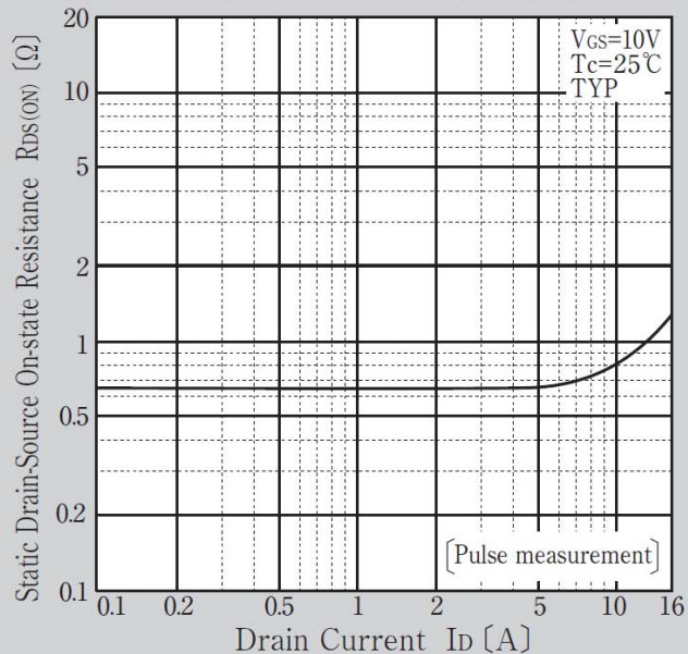
Static Drain-Source On-static Resistance vs Drain Current
