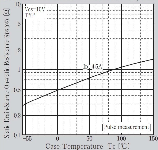
Static Drain-Source On-static Resistance vs Case Temperature
