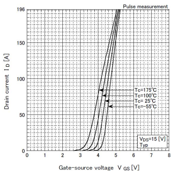
Transfer characteristics
