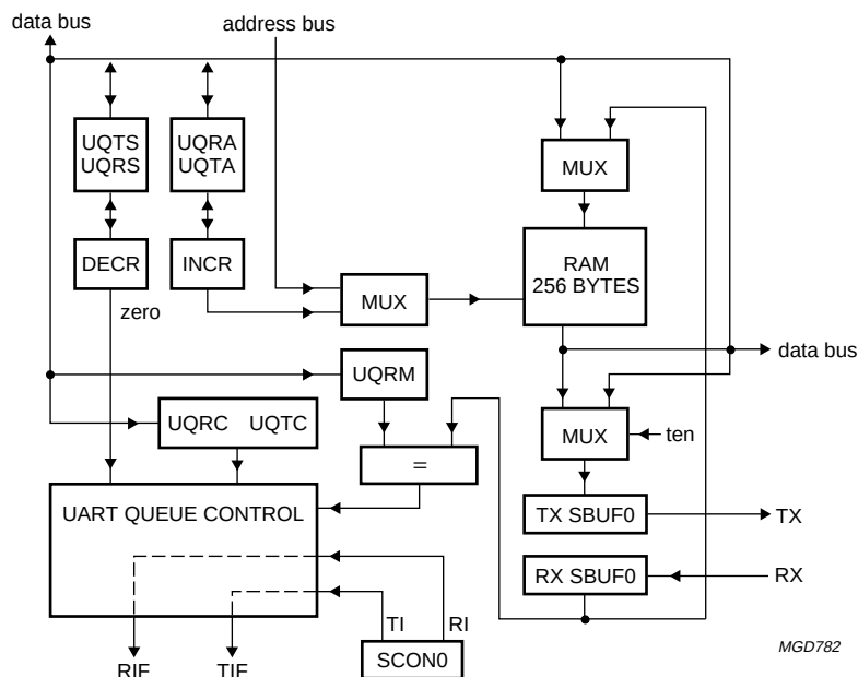
Fig.12 UART queue block diagram.
