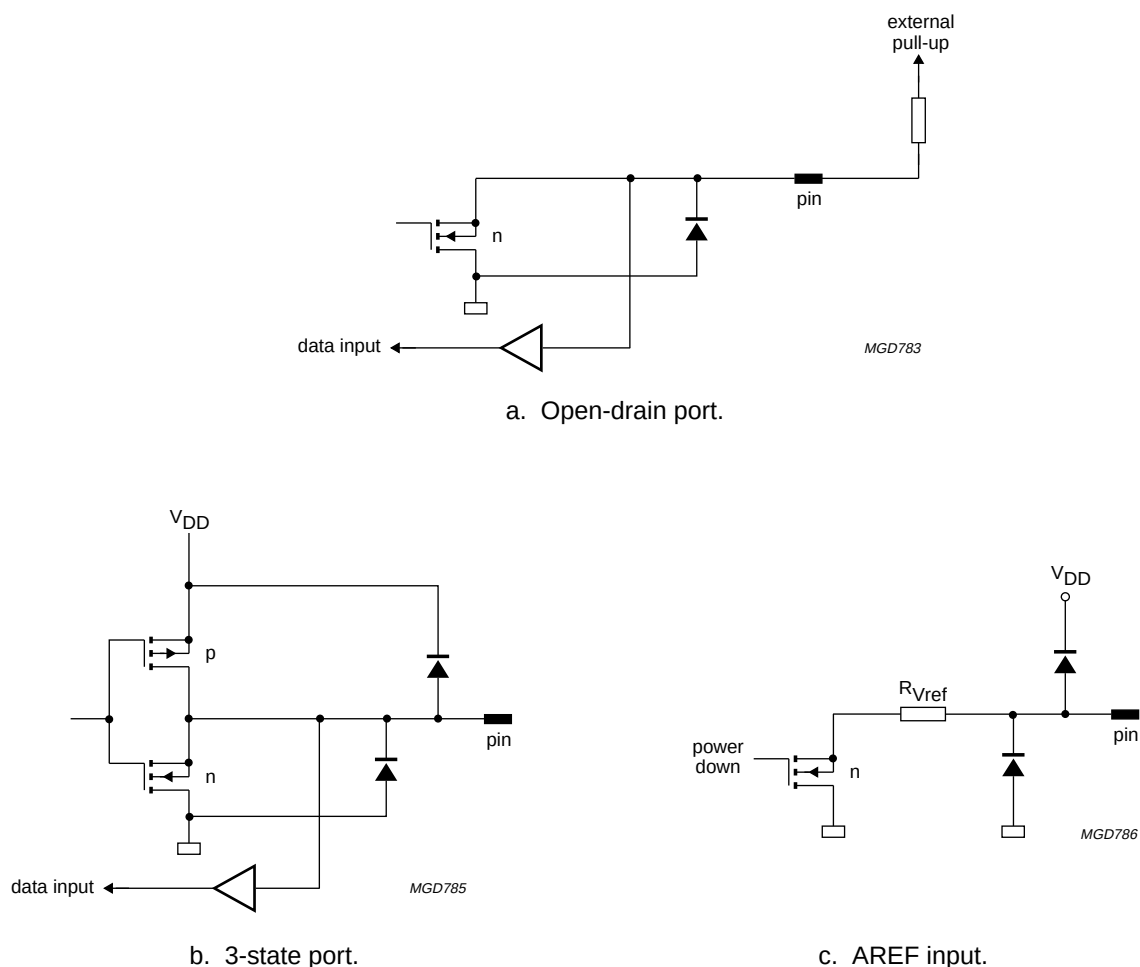
Fig.9 Port schematics (continued from Fig.8).
