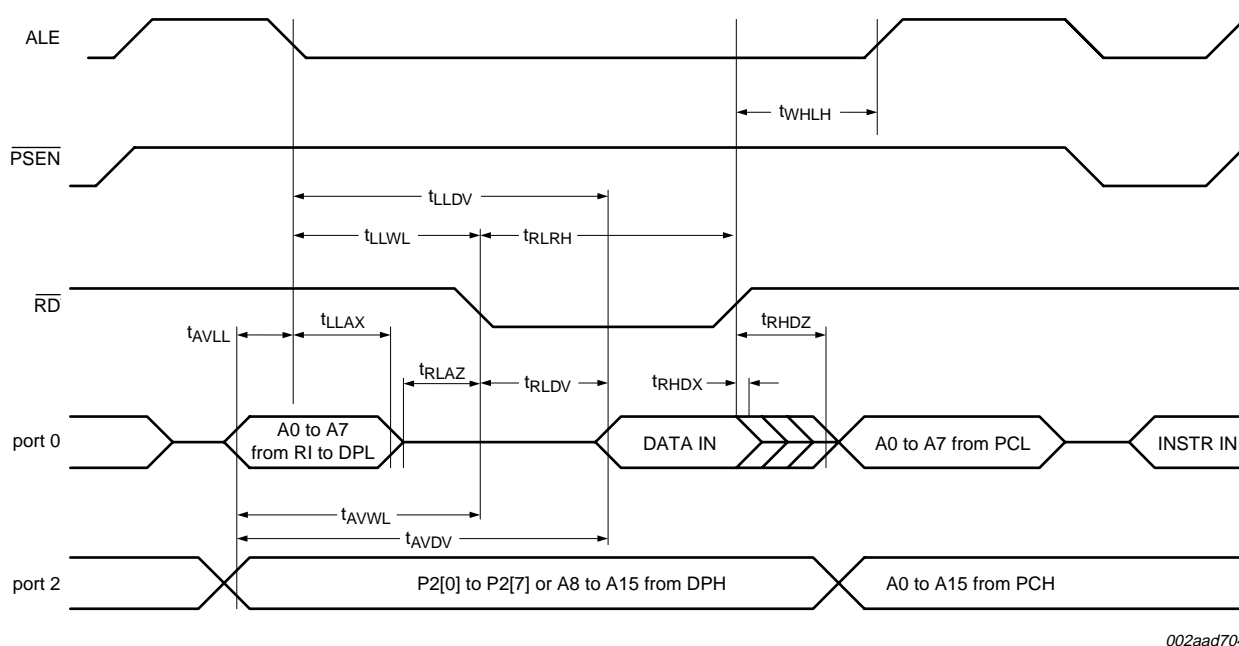
Fig 22. External data memory read cycle
