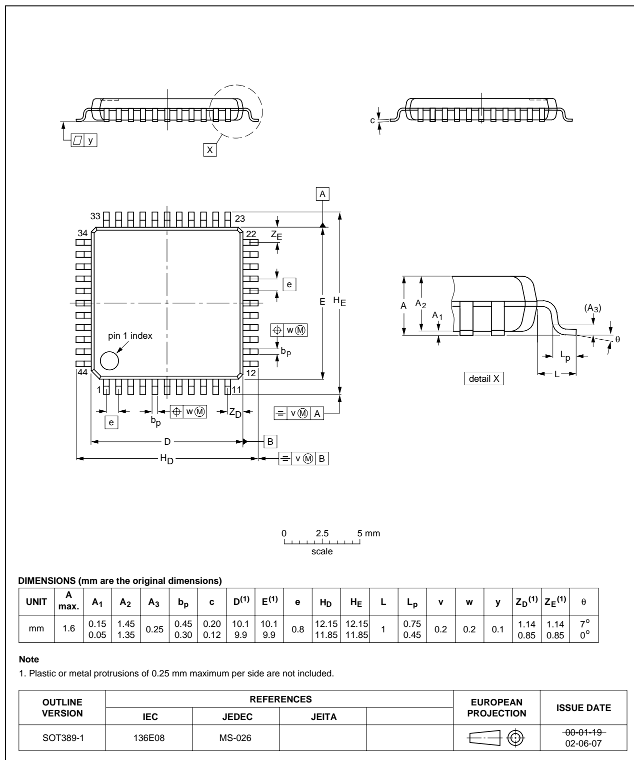
Fig 31. Package outline SOT389-1 (LQFP44)
