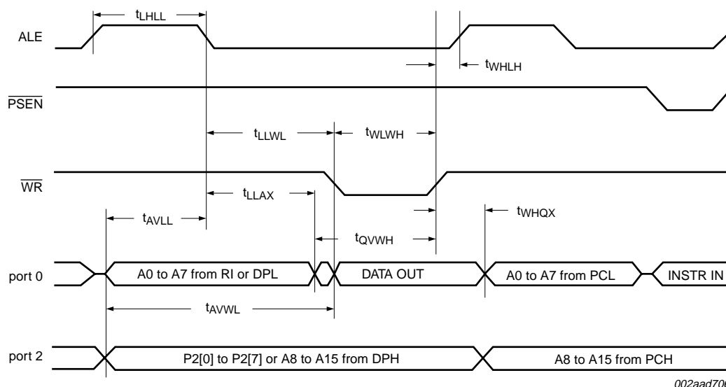
Fig 23. External data memory write cycle
