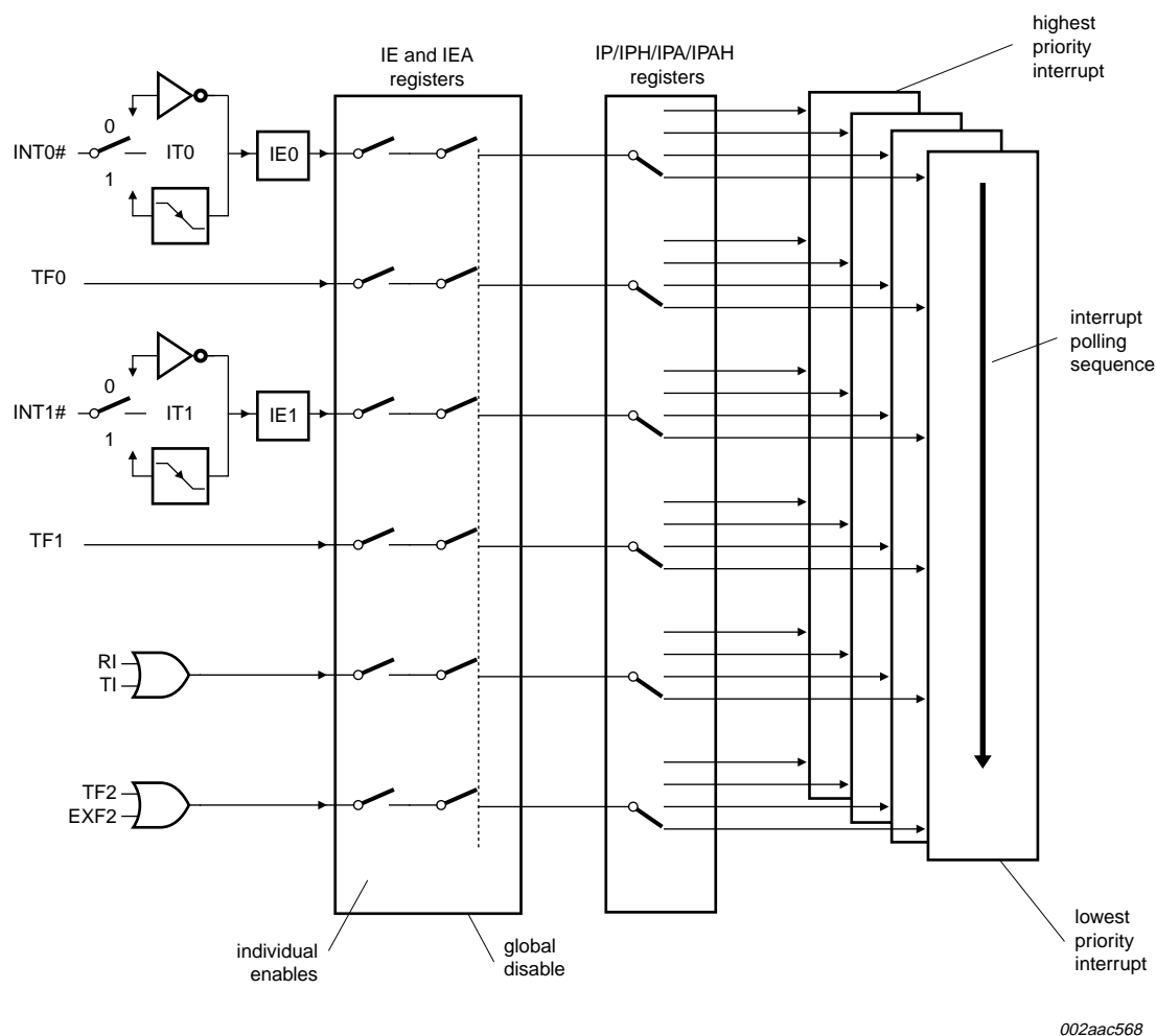
Fig 19. Interrupt structure
