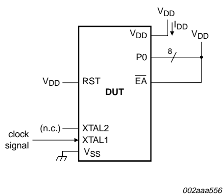
Fig 27. I_{DD} test condition, active mode
