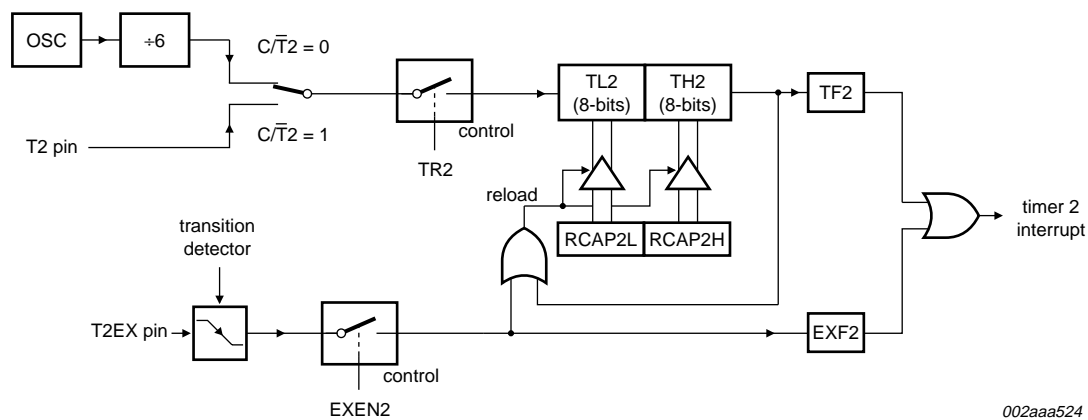
Fig 15. Timer 2 in auto-reload mode (DCEN = 0)
