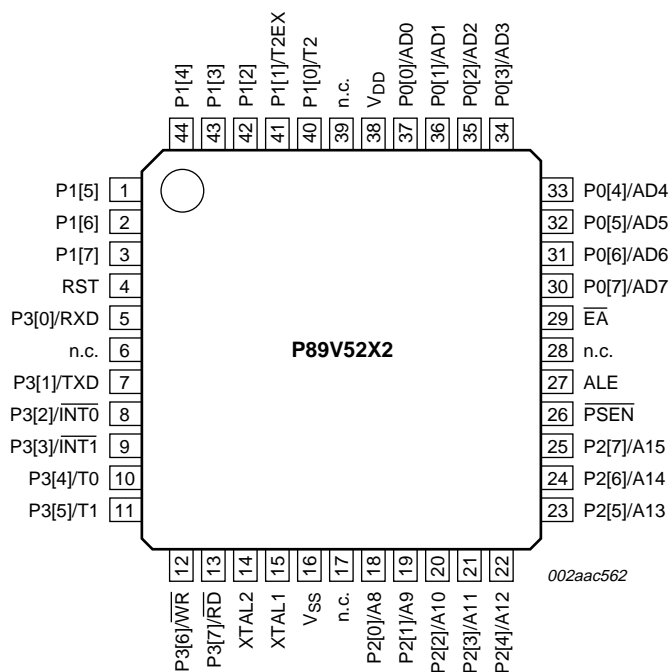
Fig 4. LQFP44 pin configuration
