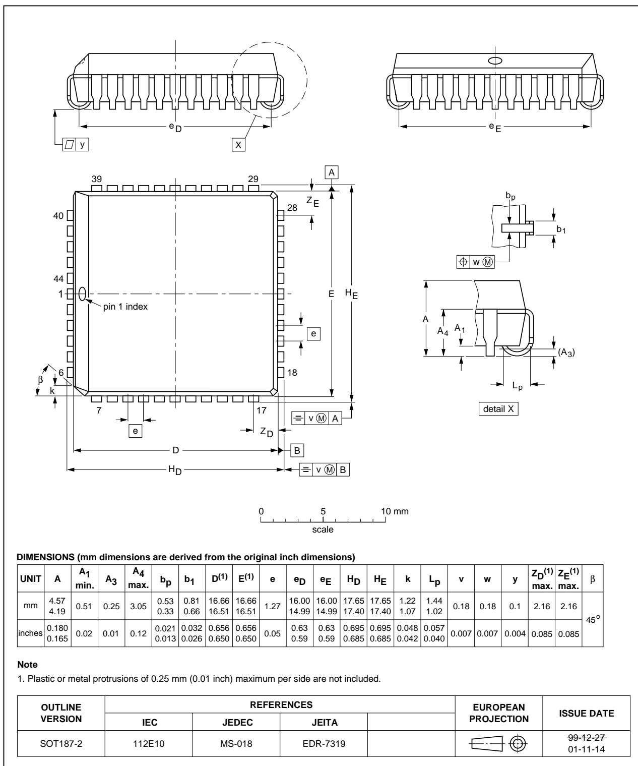
Fig 32. Package outline SOT187-2 (PLCC44)
