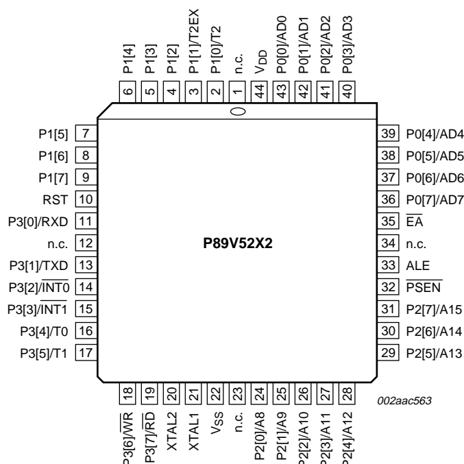
Fig 3. PLCC44 pin configuration
