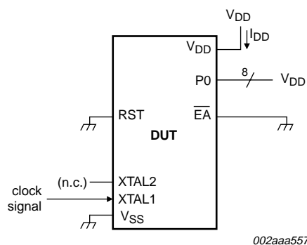
Fig 28. I_{DD} test condition, Idle mode
