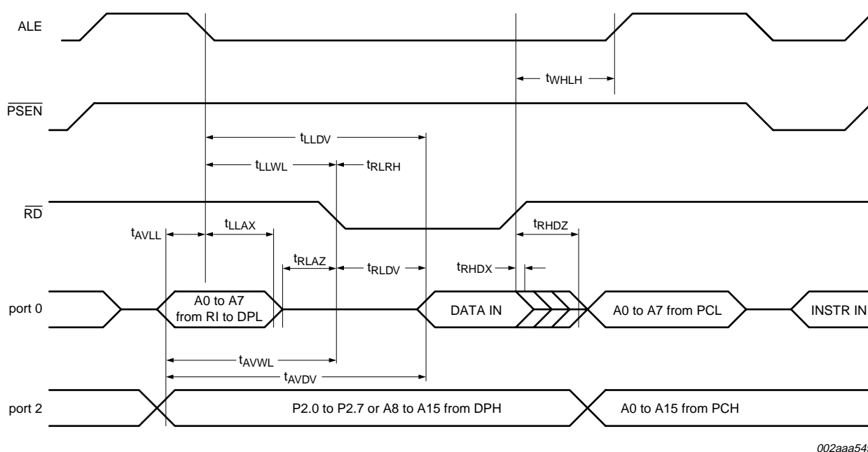
Fig 30. External data memory read cycle
