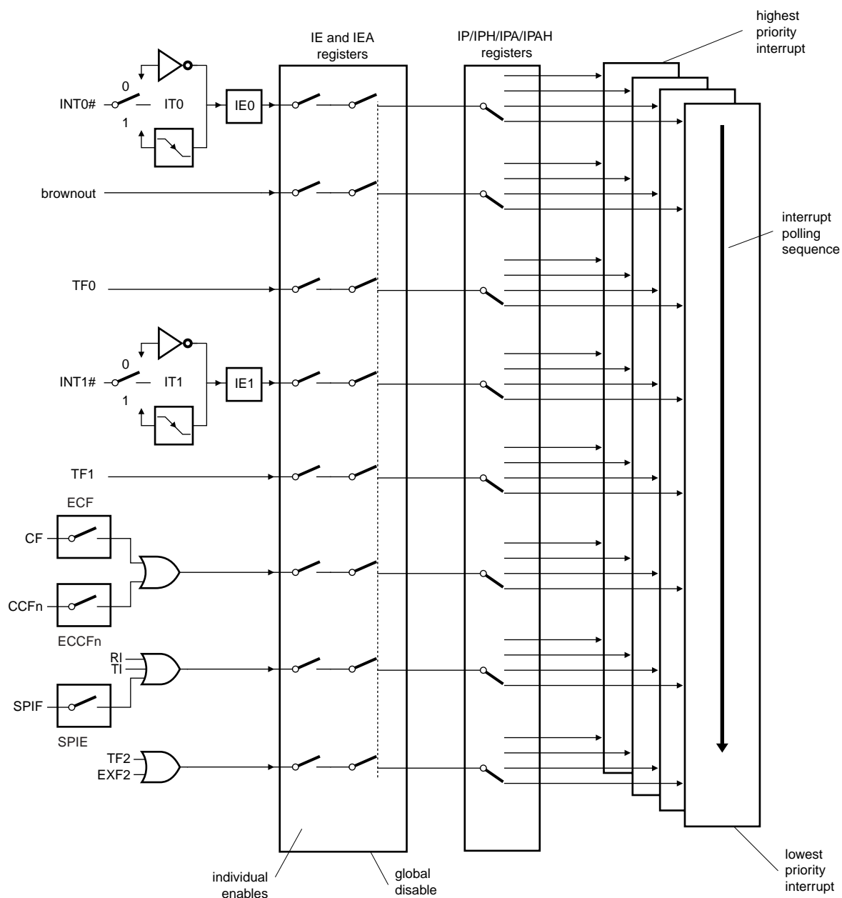
Fig 26. Interrupt structure
