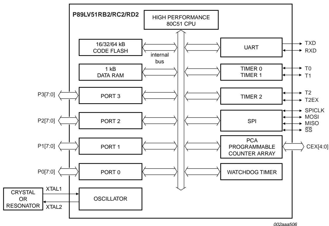
Fig 1. Block diagram
