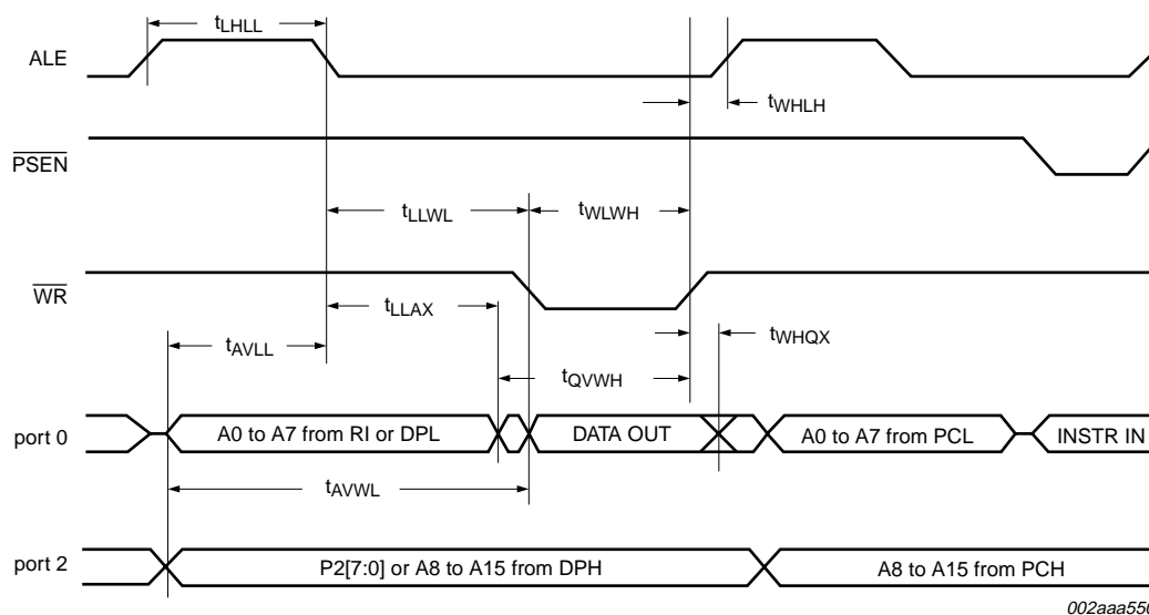
Fig 31. External data memory write cycle
