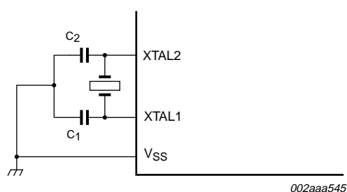
On-chip oscillator
