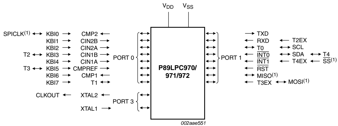
Fig 2. Functional diagram
