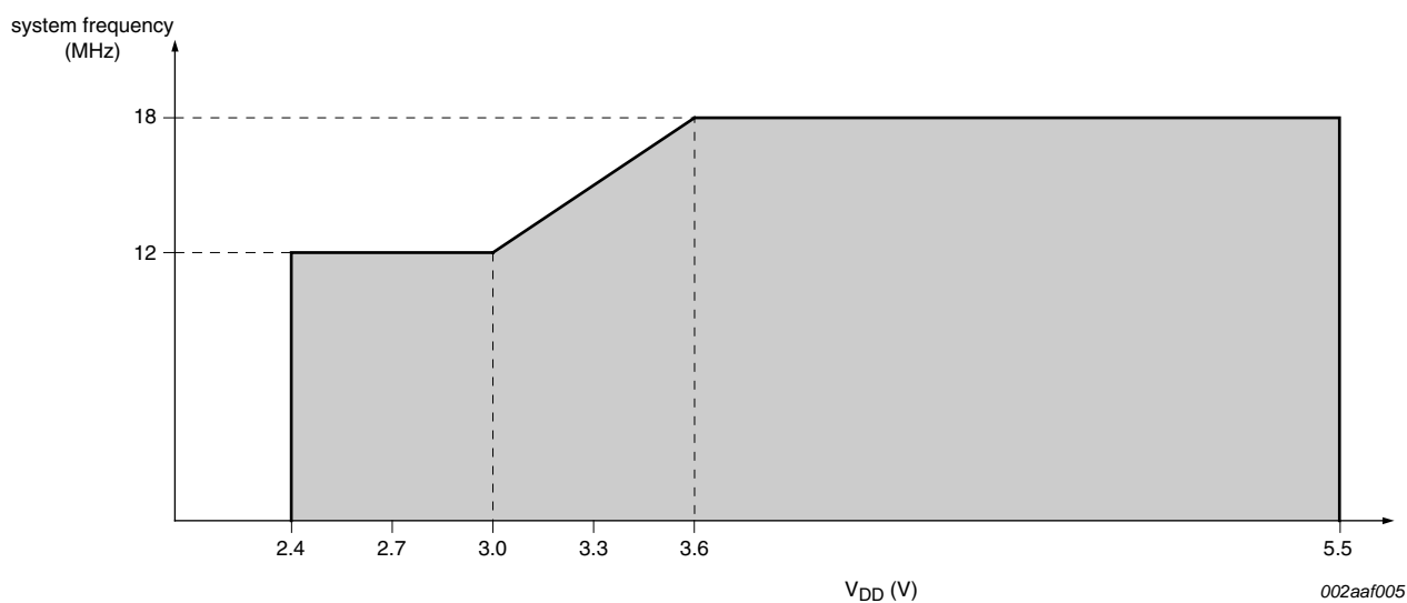
Fig 16. Frequency vs. supply voltage
