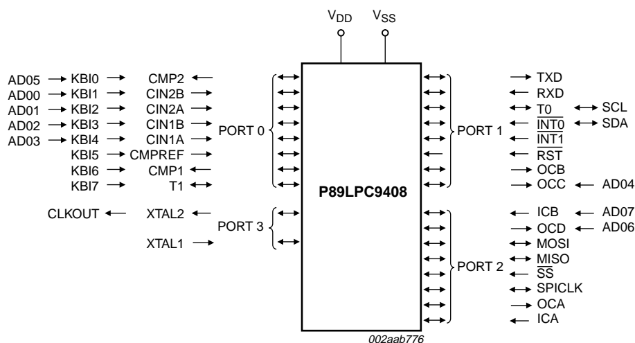
Fig 4. P89LPC9408 functional diagram
