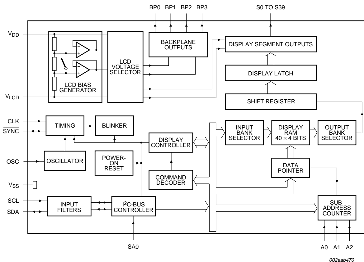
Fig 3. LCD display controller block diagram
