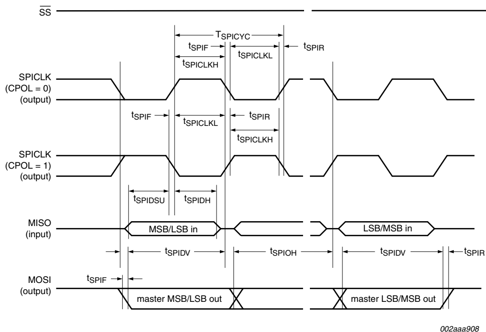
Fig 19. SPI master timing (CPHA = 0)
