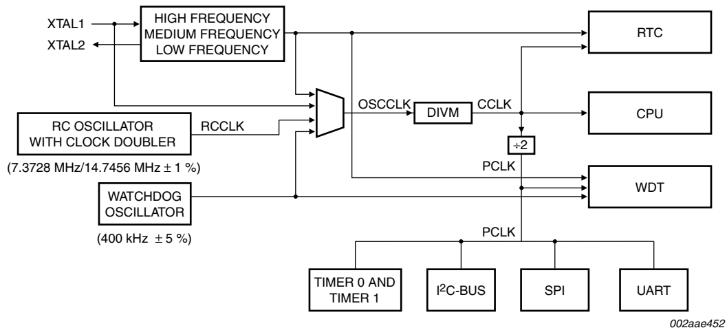
Fig 6. Block diagram of oscillator control - P89LPC9402
