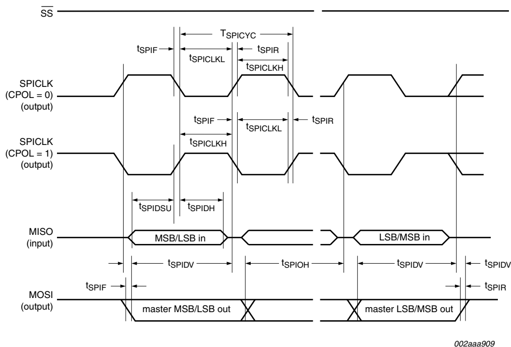
Fig 20. SPI master timing (CPHA = 1)
