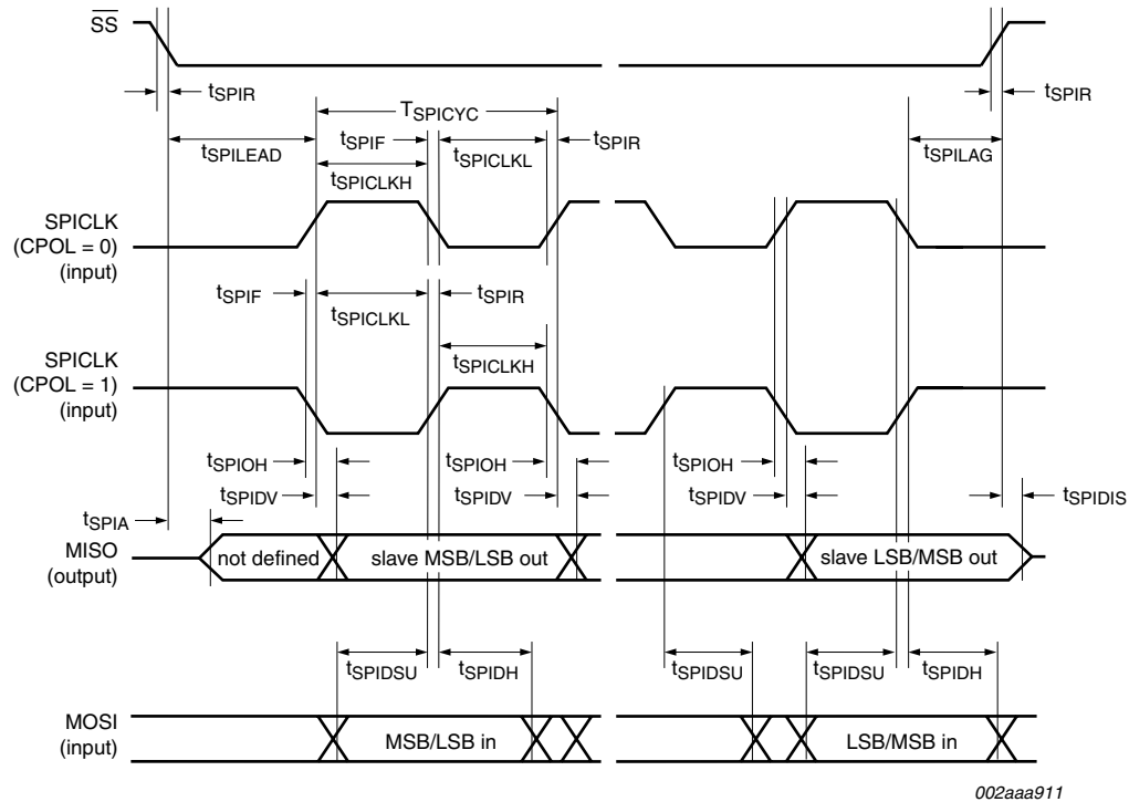
Fig 22. SPI slave timing (CPHA = 1)
