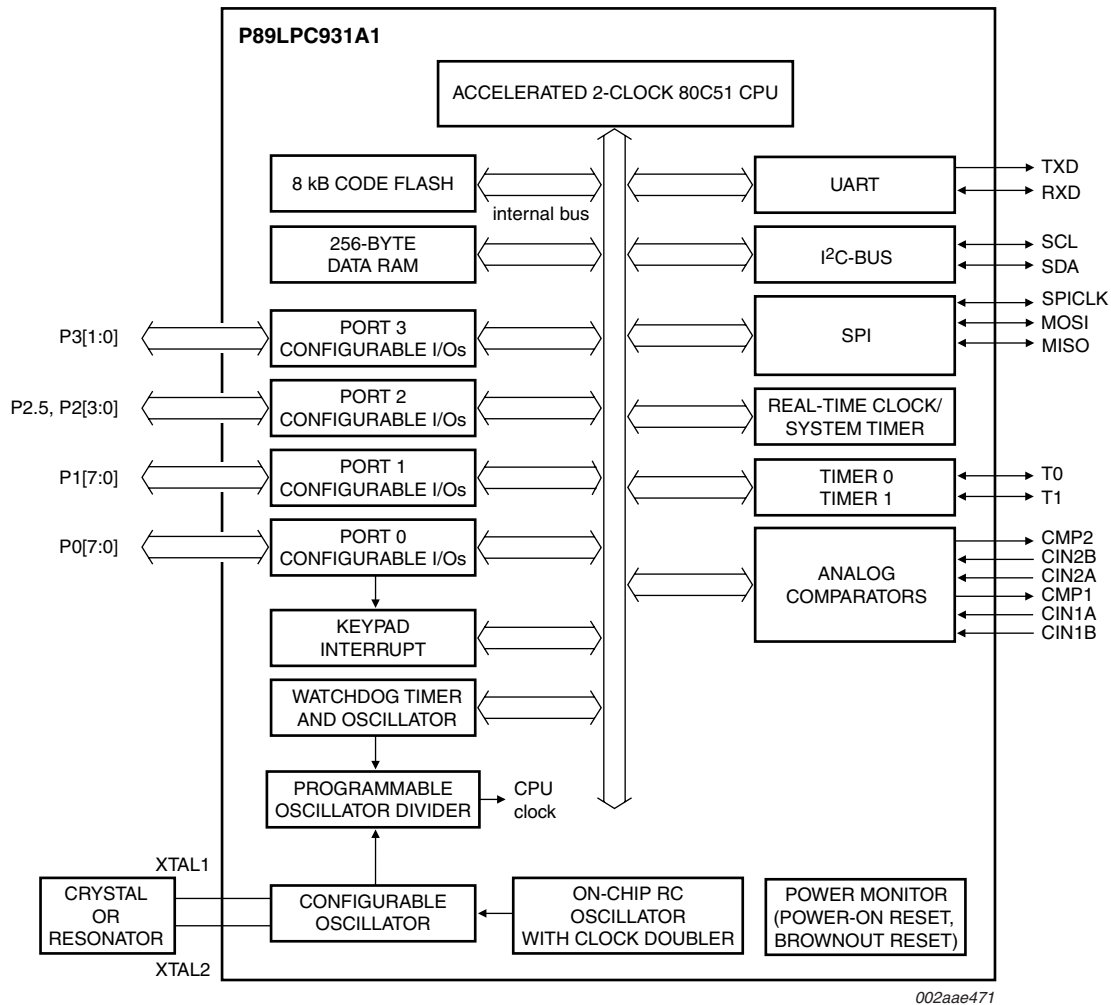
Fig 2. Microcontroller section block diagram
