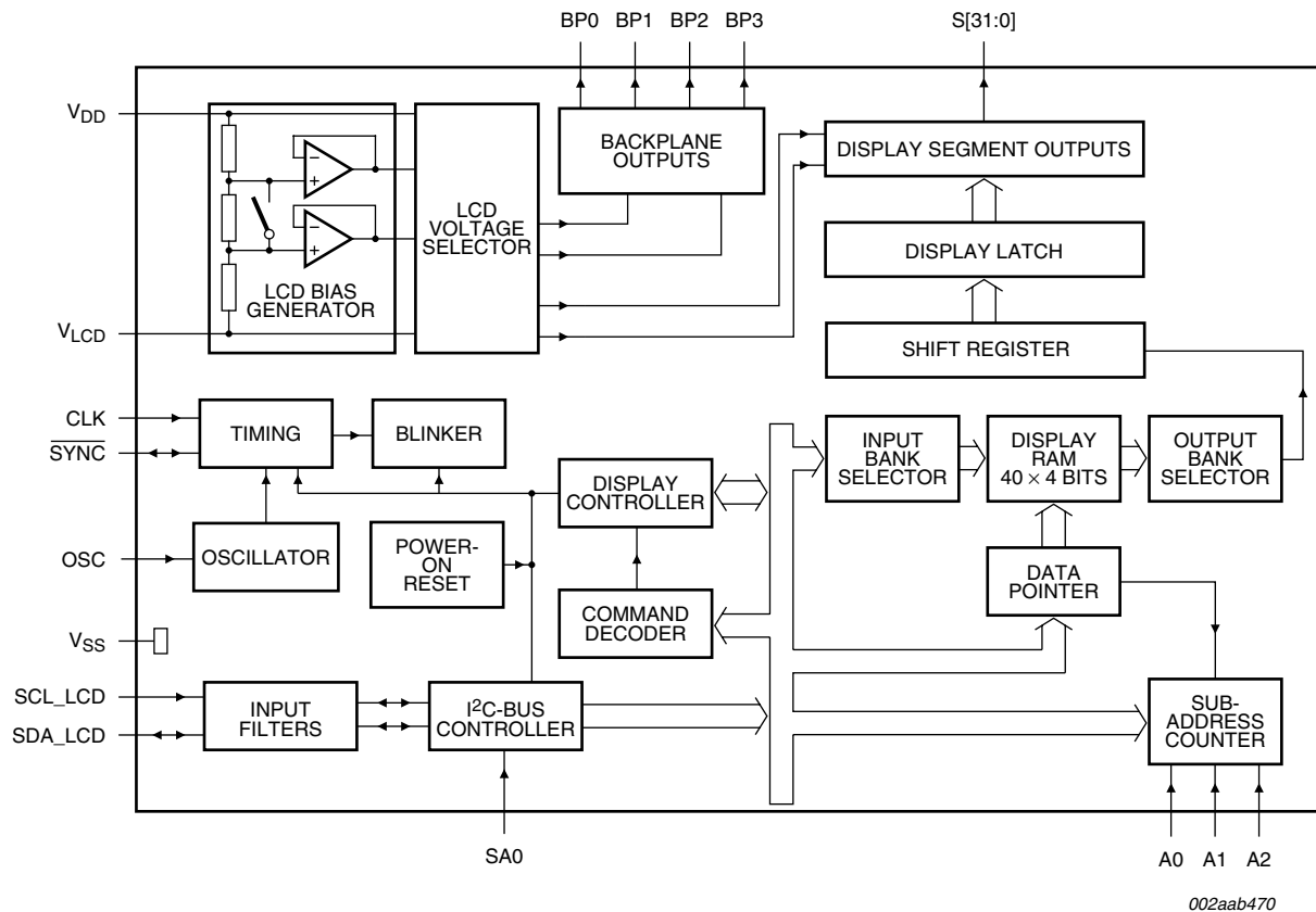
Fig 3. LCD display controller block diagram
