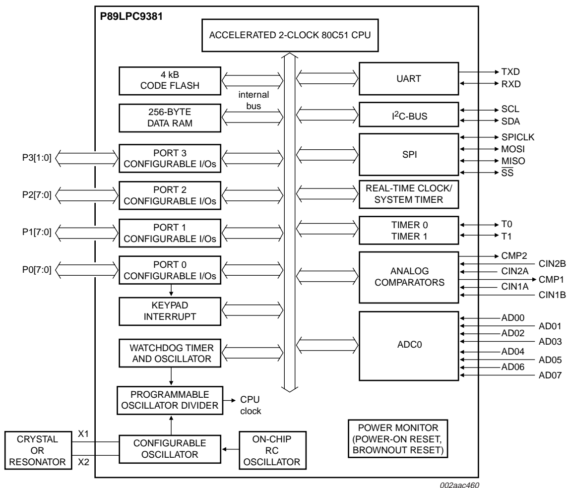
Fig 1. Block diagram
