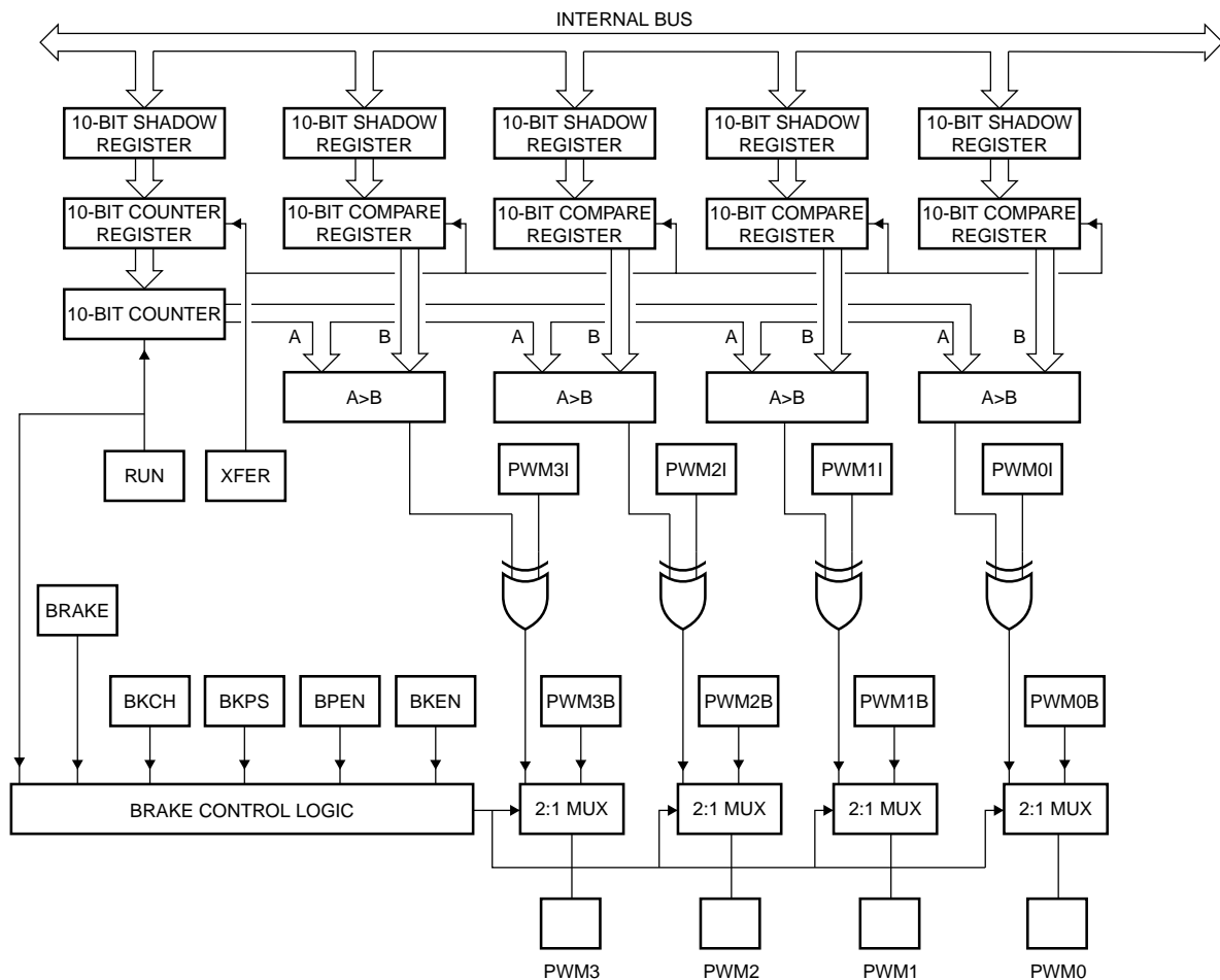
Fig 8. PWM block diagram.
