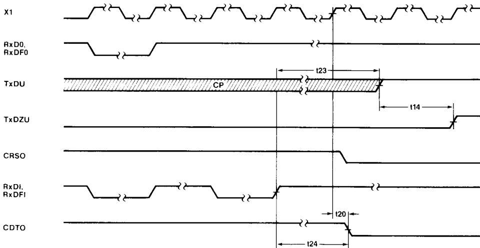
(b) END OF COLLISION
