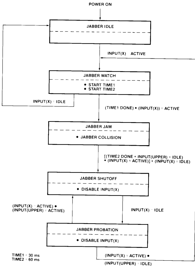
Figure 4. Jabber Timer State Diagram
