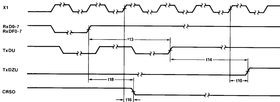
(b) END OF FRAME
