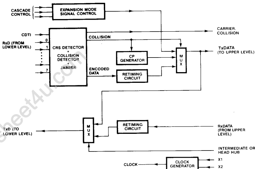
Figure 1. 82C551 Hub Block Diagram
