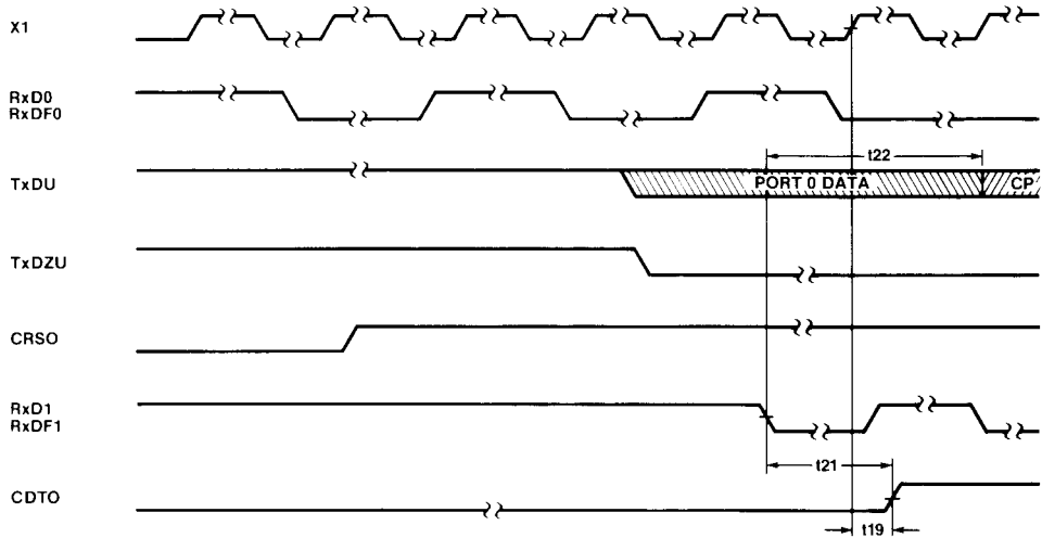
(a) START OF COLLISION
