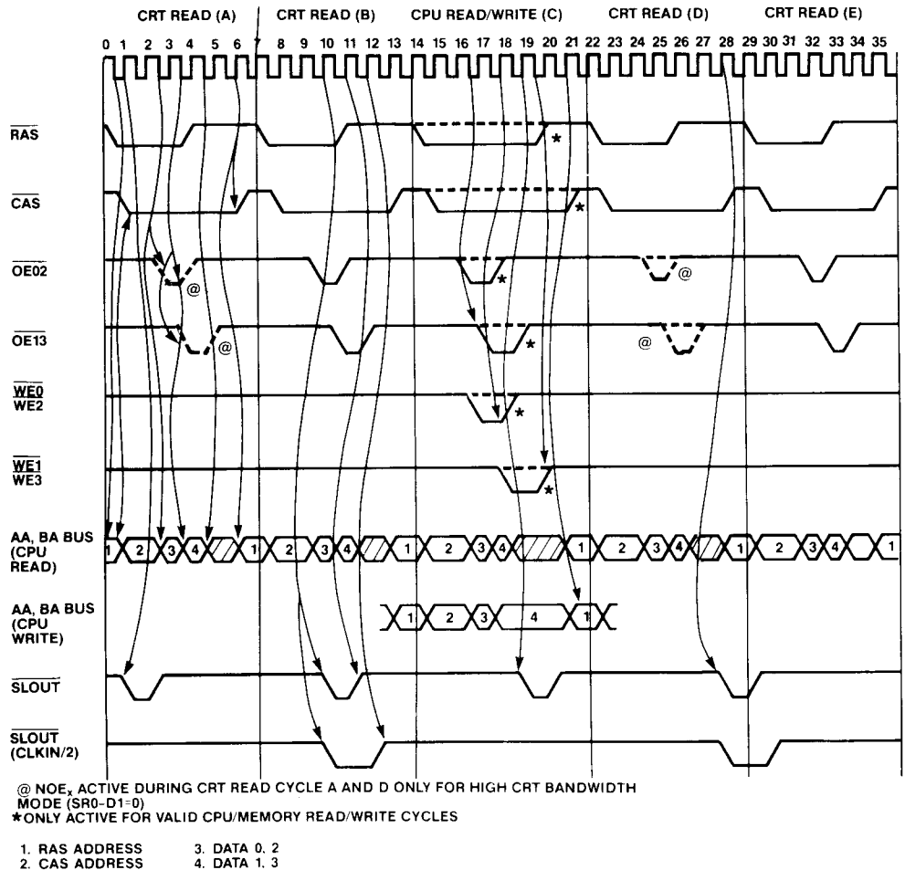
Figure 7. Memory Cycle Division for Low CRT Bandwidth Mode (SR1-D5=0), 9 Dots/Character
