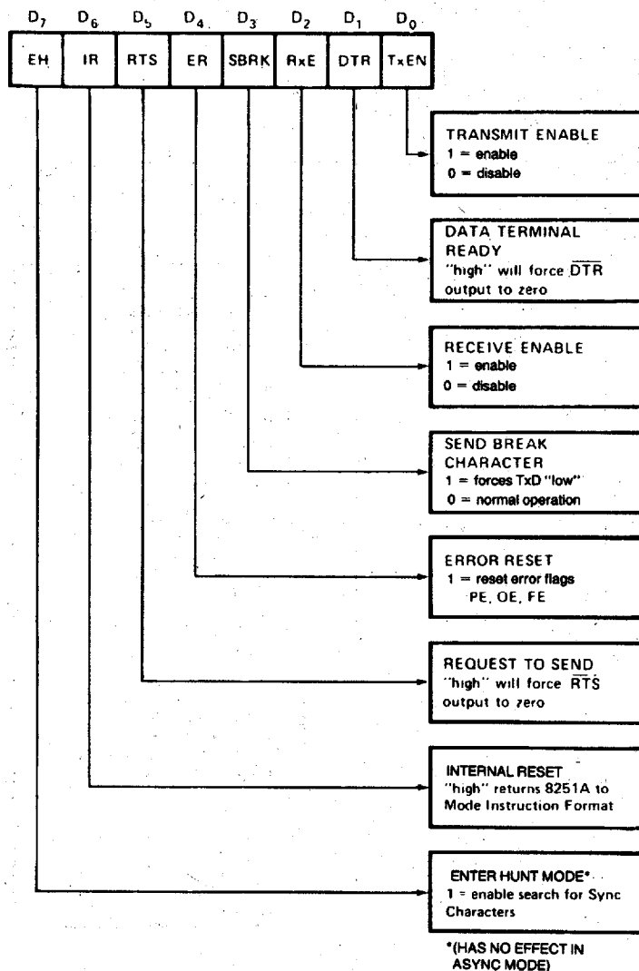
Figure 12. Command Instruction Format
