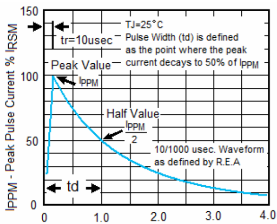
Fig. 3 Pulse Waveform
