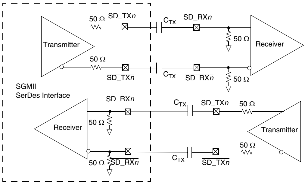
Figure 48. 4-wire AC-coupled SGMII serial link connection example
