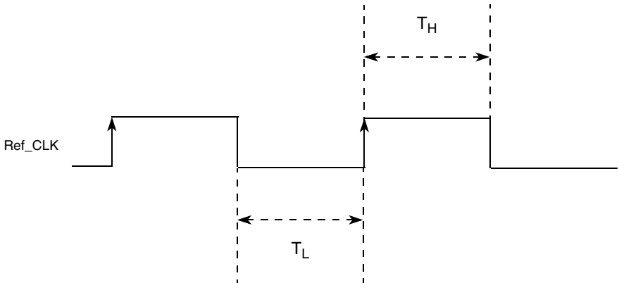
Figure 47. Reference clock timing waveform
