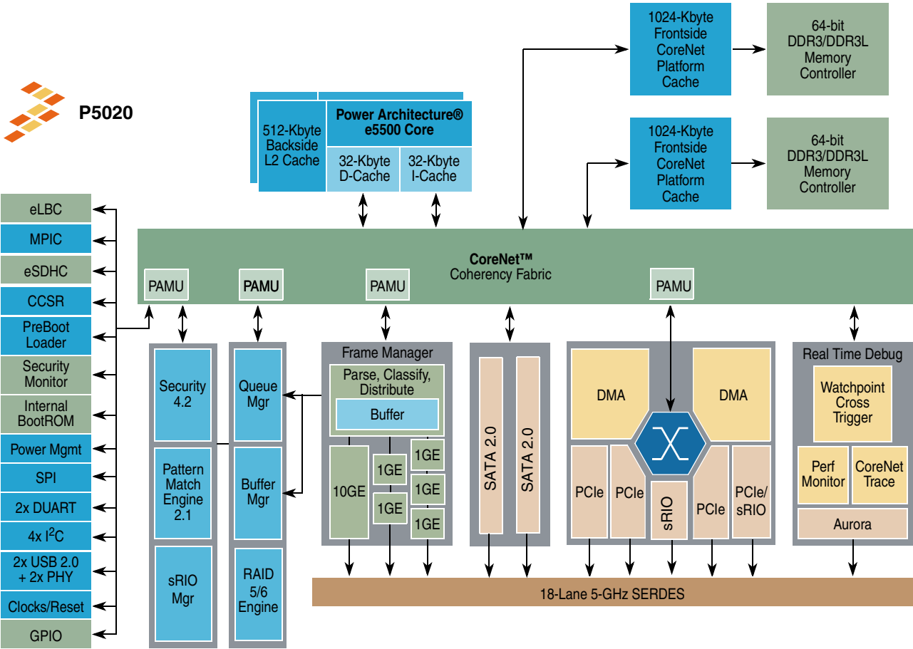
Figure 1. Preliminary P5020 block diagram
