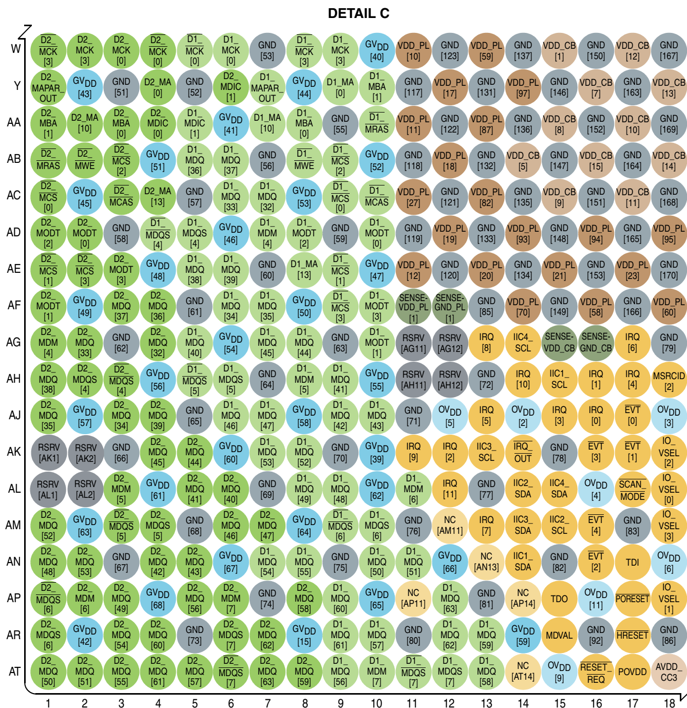
Figure 6. P5020—1295 BGA ball map diagram (detail view C)
