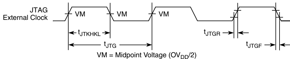
Figure 30. JTAG clock input timing diagram
