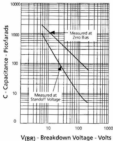
FIGURE 3 P4KE Typical Capacitance vs Breakdown Voltage (Unipolar)
