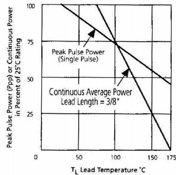
FIGURE 1 Derating Curve
