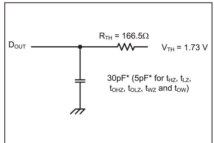
Figure 2. Thevenin Equivalent
