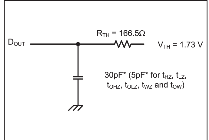
Figure 2. Thevenin Equivalent
