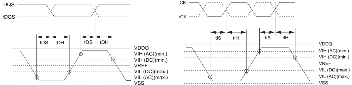
Input Waveform Timing 1 (tDS, tDH)
