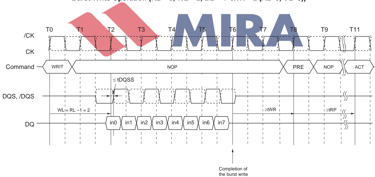
Burst Write Operation (RL = 3, WL = 2, BL = 8 (AL=0, CL=3))
