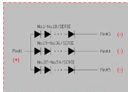
Connector :CN3(CI1605M1VRA-NH)
