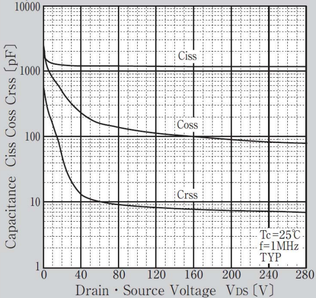
Capacitance Characteristics
