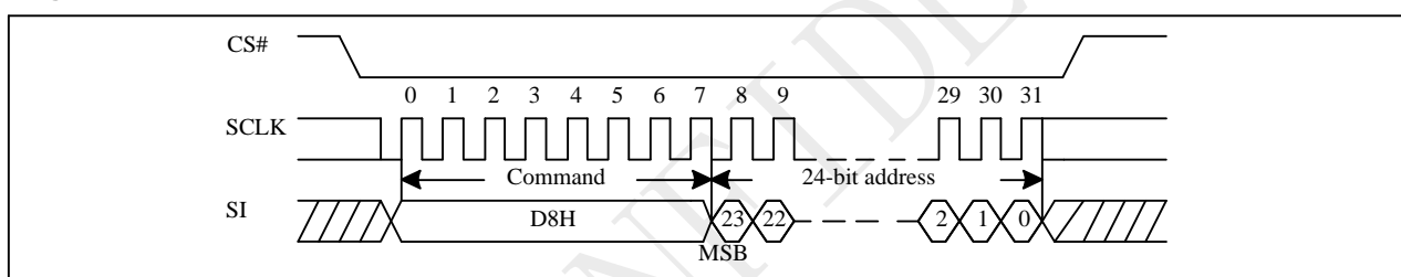
Figure 10-30 Block Erase (BE) Sequence (Command D8)
